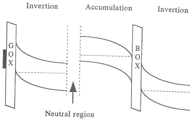
Figure 8.b. Energy band diagram of the MISIS structure under reverse bias voltage.
