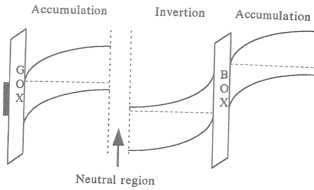
Figure 8.a. Energy band diagram of the MISIS structure under forward bias voltage.
