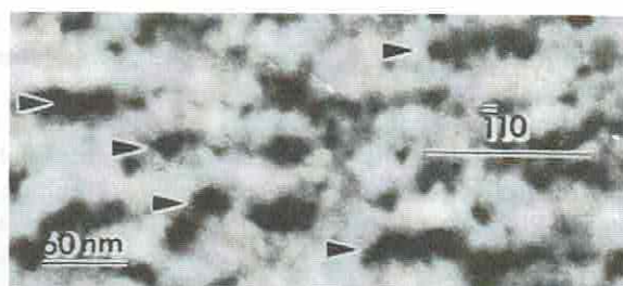
FIG. 3. Plan-view bright-field TEM image ( g=220 ) of 3.3-ML \text{In}_{0.5}\text{Ga}_{0.5}\text{As} grown at 320^\circ\text{C} .
