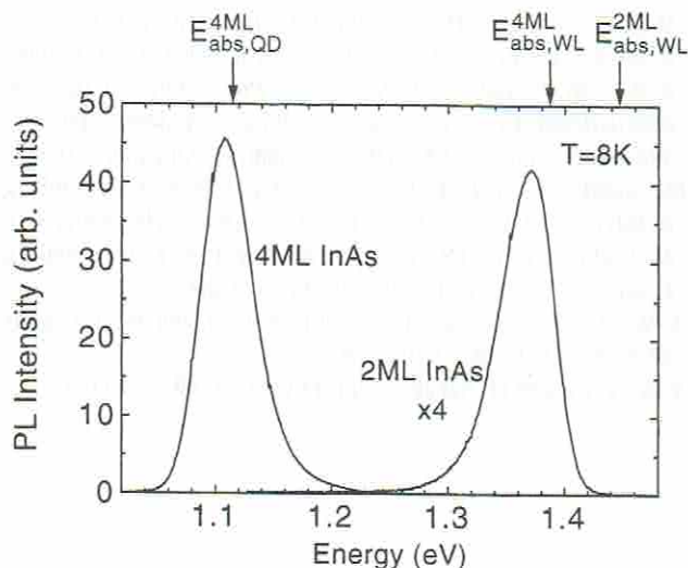
FIG. 4. Low-temperature ( T=8\text{ K} ) PL spectra of quantum dots in samples with 2 and 4 ML of InAs at excitation density D=1\text{ W cm}^{-2} . The peak energies in the absorption spectra for the wetting layer (WL) in both samples and the quantum dots in the 4-ML sample are shown by arrows.
